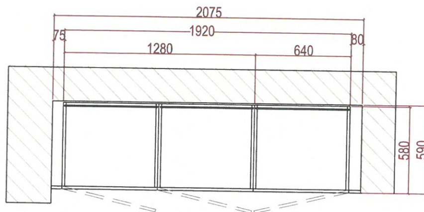
KIDS ROOM WARDROBE-LAYOUT
