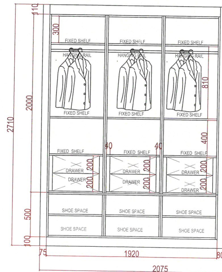
KIDSROOM WARDROBE- INNER VIEW
