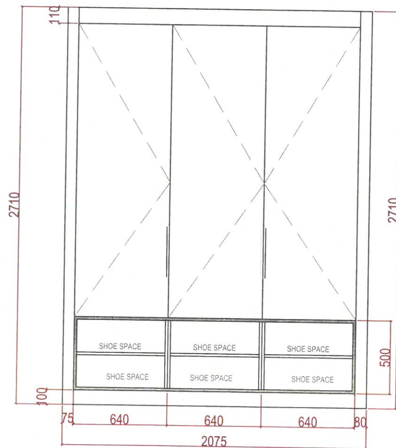
KIDSROOM WARDROBE- FRONT VIEW
